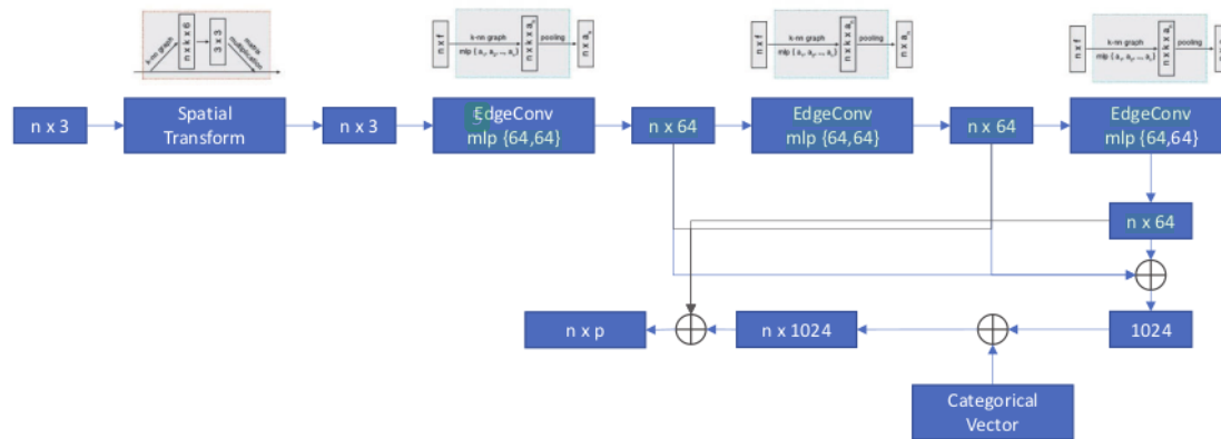
Fig. 3. DGCNN architecture.
