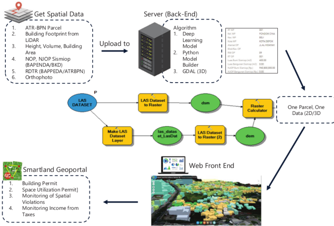
Fig. 2. Smart Land Surveillance (SLSS) business process.
