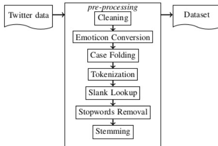
Fig. 1. The pre-processing steps.
