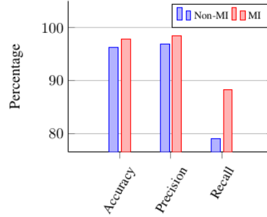
Fig. 7. The average accuracy, precision, and recall of the MI feature existent.
