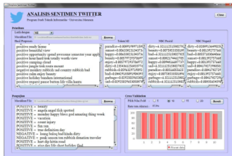
Fig. 9. The system user interface.
