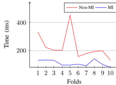
Fig. 8. The classification time variation of the MI feature existent.
