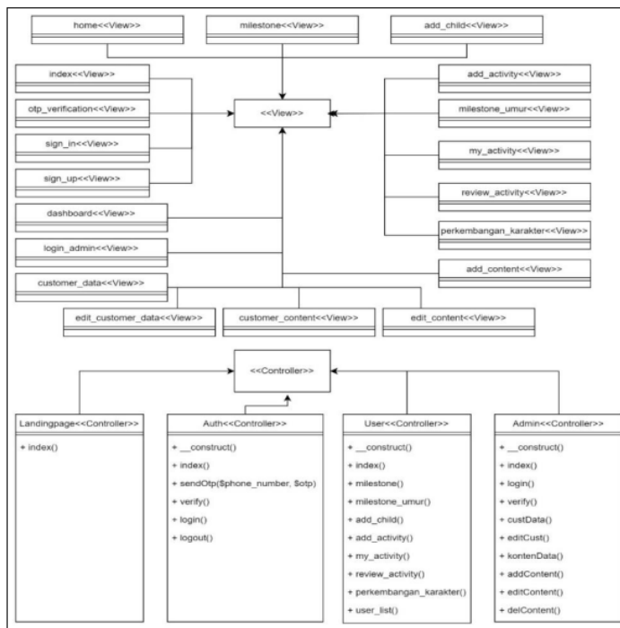
Gambar 3. Class diagram
