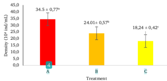
Figure 2. Population density of the microalgae at the peak phase. Different superscripts showed significant differences.
