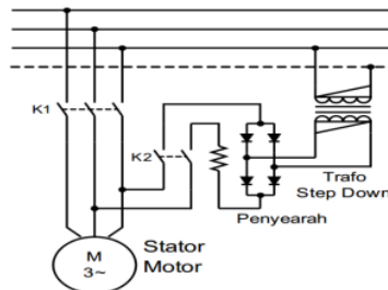
Gambar 2. Diagram Dinamik Braking (Warsito, 2006)
