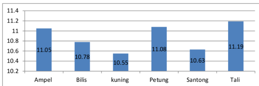
Gambar 3. Rerata Nilai Rata-rata Kadar Air Kering Udara Bambu di Kawasan KHDTK Senaru
