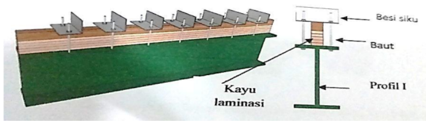
Gambar 1. Model Pengempaan balok laminasi (Rahmalia, 2016) Figure 1. Laminate beam compression model (Rahmalia, 2016)
