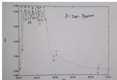
Figure 7. UV-vis anacardic acid spectrum
