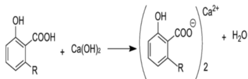
Figure 2. The reaction of anacardate calcium salt formation.
