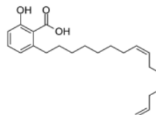
Figure 1. The general structure of c
