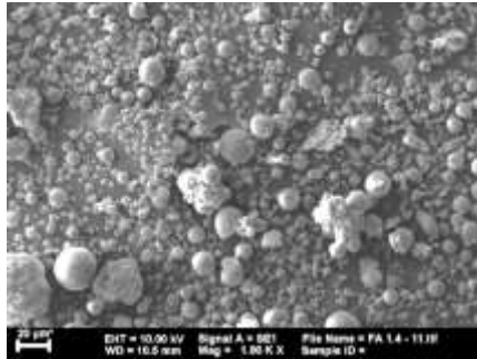
Fly ash (1,000X)
