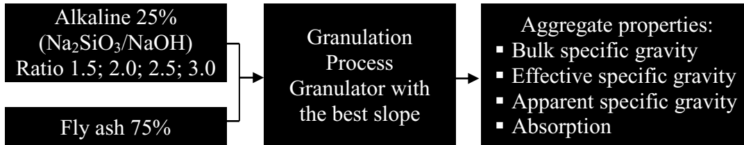
Fig 4. Experiment to find the best alkaline ratio
