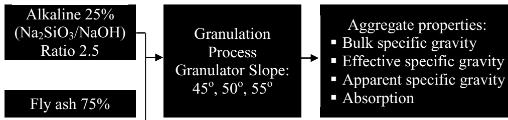
Fig 3. Experiment to find the best slope [11]
