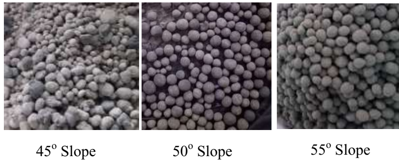
Fig 5. Artificial aggregates with \text{Na}_2\text{SiO}_3/\text{NaOH} ratio of 2.5 and slope variations [11]
