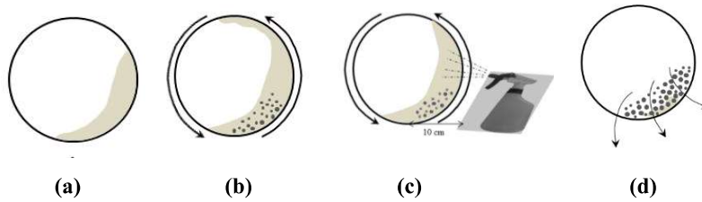
Fig. 1. Manufacturing process of artificial geopolymer aggregates.
