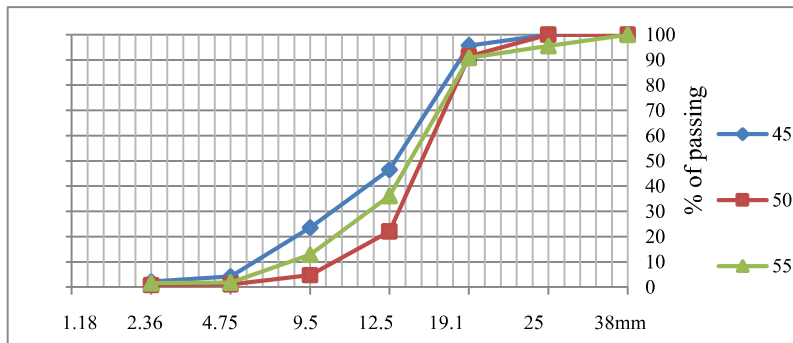
Fig. 3. Artificial geopolymer aggregate gradation.
