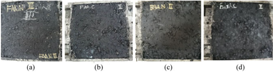
Fig. 5 Four asphalt mixture sample sets: a dense graded without artificial aggregate, b dense graded with 25% artificial aggregate, c open graded without artificial aggregate, d open graded with 25% artificial aggregate
