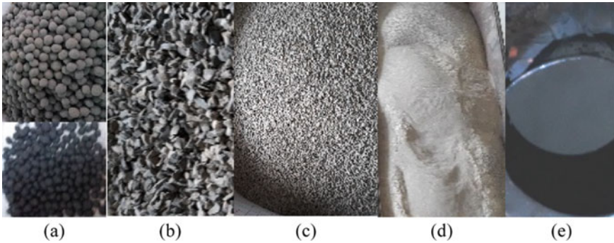
Fig. 2 a Artificial aggregate, b coarse aggregate, c fine aggregate, d filler, and e bitumen
