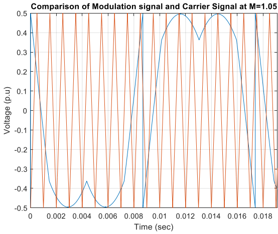
Fig. 5. Comparison of modulation signal and the carrier signal
