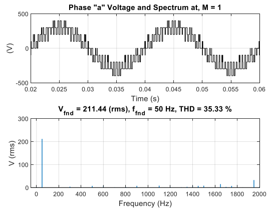
Fig. 8. Inverter phase 'a' output voltage at M = 1.0
