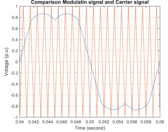
Fig. 4. Comparison of modulation signal and the carrier signal
