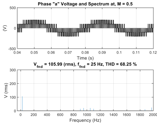
Fig. 9. Inverter phase 'a' output voltage at M = 0.5
