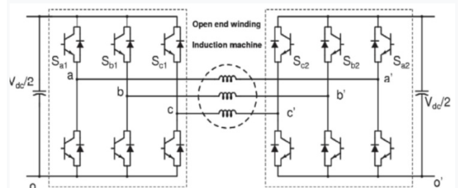
Fig. 1. Dual inverter fed open-end winding motor structure [9]
