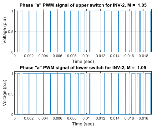
Fig. 7. Phase 'a' PWM signal of dual inverter fed structure for inverter -2
