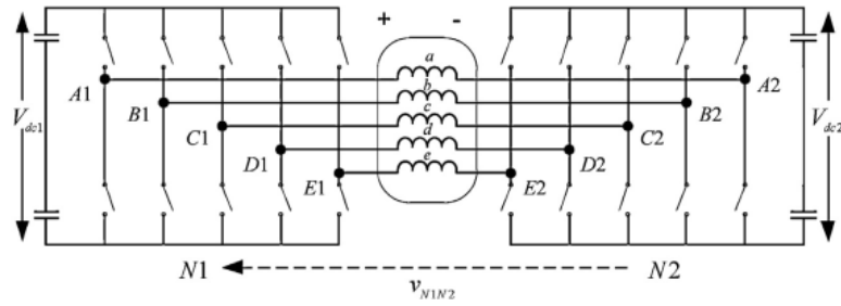
Fig. 3. Five-phase machine with dual two-level inverter supply.
