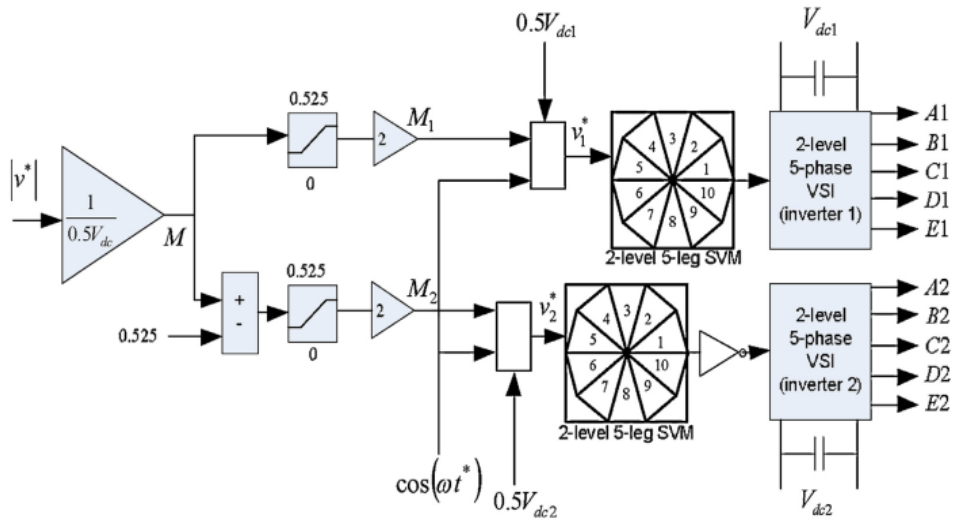
Fig. 5. Unequal reference sharing scheme.
