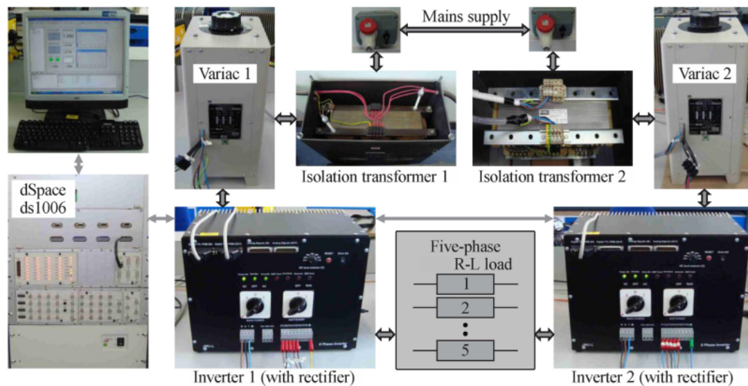
Fig. A1. A1 Experimental setup of the open-end winding five-phase supply topology.
