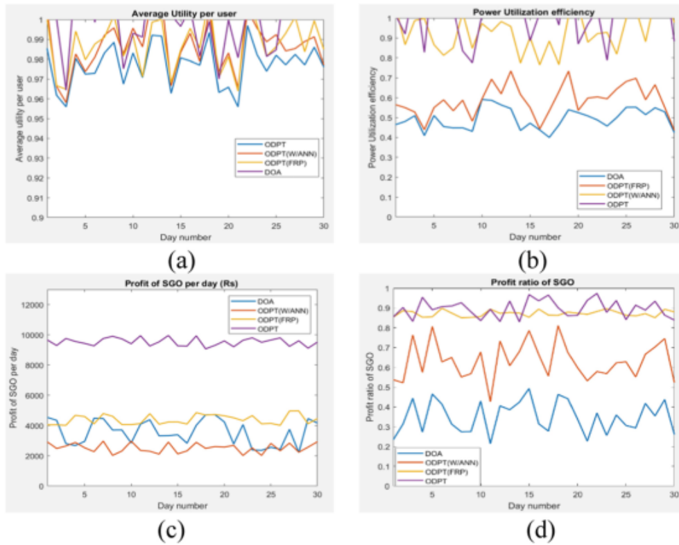
Fig. 4. Figure showing (a) Average User Utility, (b) Power Utilization Efficiency, (c) Per day profit of SGO, and (d) Profit ratio of SGO.
