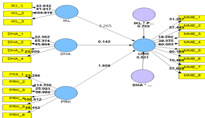
Figure 4. Resampling Bootstrapping Methode Output
