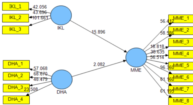
Figure 3. Bootstrapping Resampling Method Output
