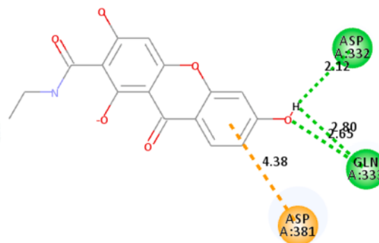
Fig. 5. 2D and 3D predicted binding mode from docking simulation of 18 and 20 into the active site of MTB C171Q (4C6X.pdb).
