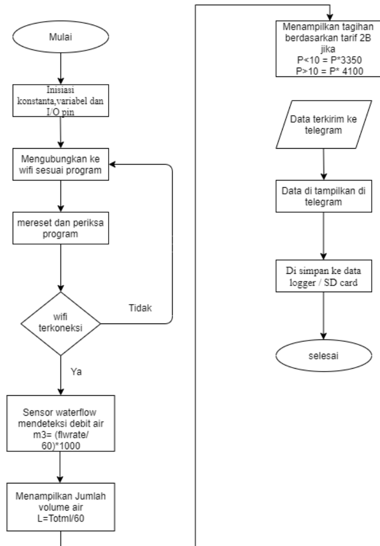
Gambar 3. Diagram Sistem
