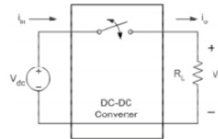
Gambar 1. Buck converter(Taufik,2008)
