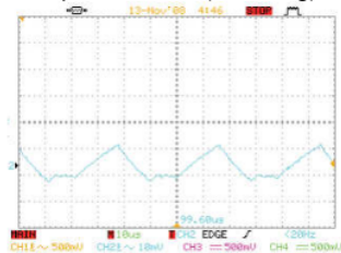
Gambar 4. Mode Discontinuous Conduction Mode (DCM) (Taufik, 2008).
