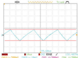
Gambar 3. Mode Continuous Conduction Mode (CCM) (Taufik, 2008).
