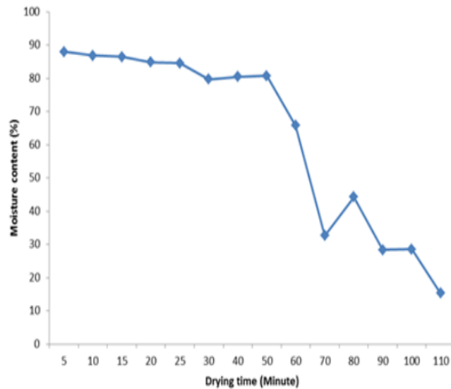
Figure 1. Moisture Content Vs Drying Time
