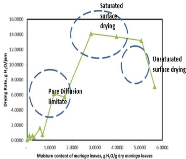
Figure 2. Graph drying rate vs moisture content
