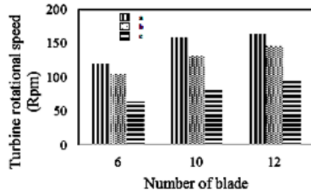
Figure 4. Effect of blade number and directional plate angle on rotational speeds, at the directional plate angles of (a) 30°, (b) 20°, (c) 10°.
