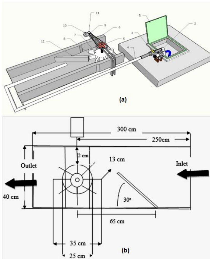
4 Figure 1. Schematic diagram of the experimental apparatus; (a) layout of the apparatus, (b) the dimension of the apparatus. 1. Water reservoir, 2. Pump, 3. Valve, 4. Pipe, 5. Big pulley, 6. V-belt, 7. Runner, 8. turbine blade, 9. Generator, 10. Lamp, 11. Small pulley, 12. Directional plate.
