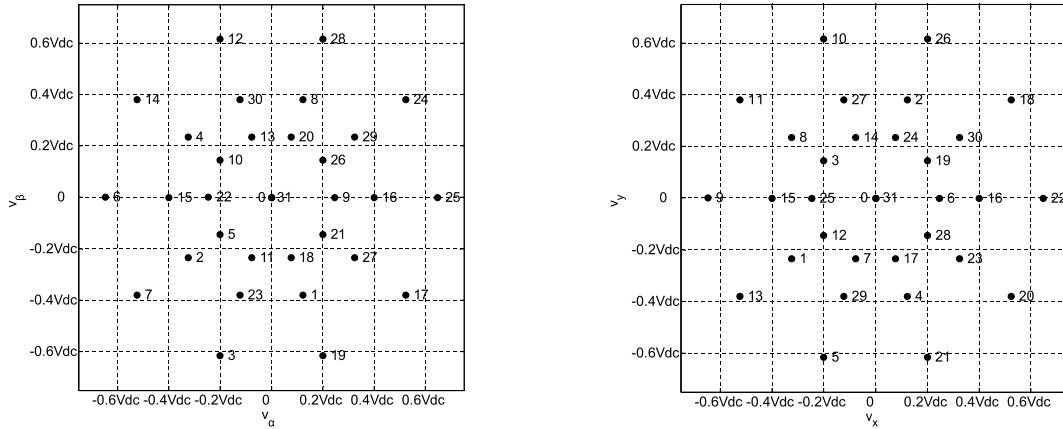
Figure 1 Two-level five-phase VSI space vectors in the \alpha\text{-}\beta and x\text{-}y planes.
