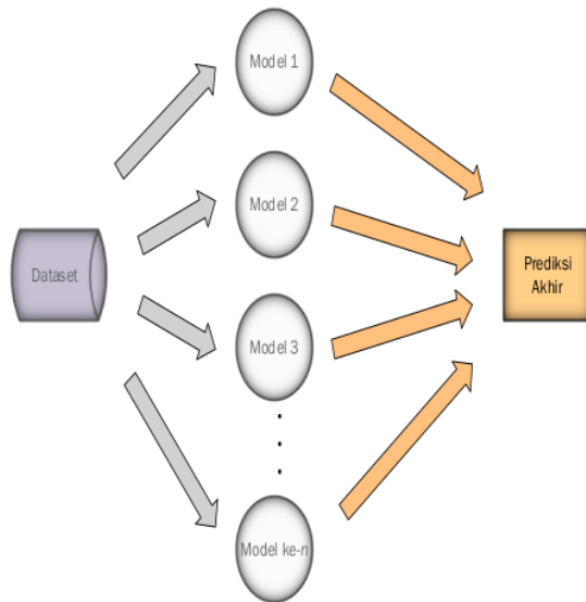
Gbr. 5 Grafik Skema Algoritma Ensemble Learning
