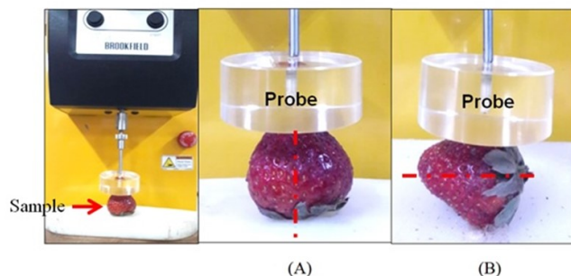
Figure 2. Strawberry fruit deformation test, (A) compression from the vertical direction, and (B) compression from the horizontal direction.
