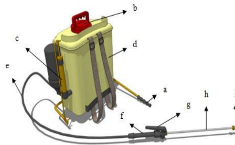
Figure 2. Knapsack sprayer type high-density polyethylene sprayer (HDPS).
