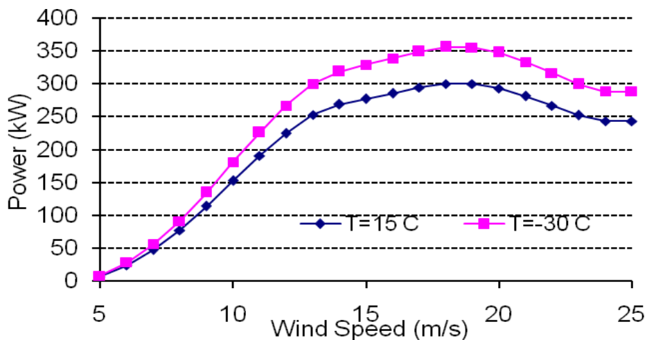
Figure 2 Comparing result power curve between temperature 15 0 C and -30 0 C
