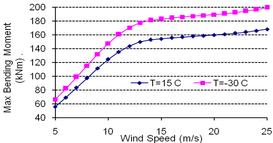
Figure 3 Comparing result of maximum bending moment at temperature 15 0 C and -30 0 C
