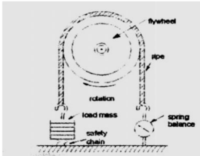
Gambar 3. Sistem Rope Brake , [5].
