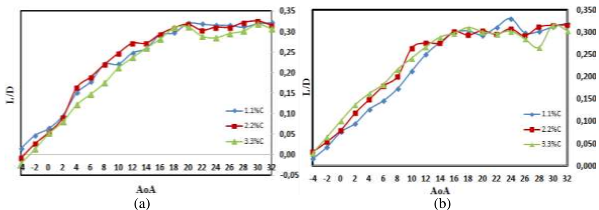
Figure 7. Comparison ratio lift and drag force of variation tab heights versus angle of attach for (a) tab upper surface and (b) tab lower surface
