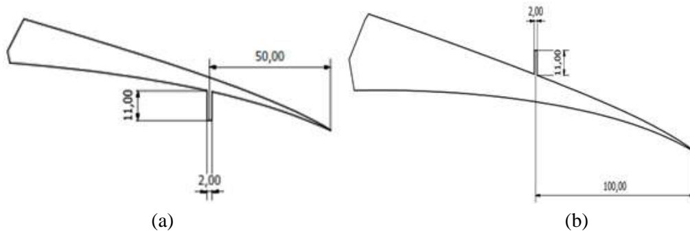
Figure 2. Detail tab location (a) tab lower surface , (b) tab upper surface.
