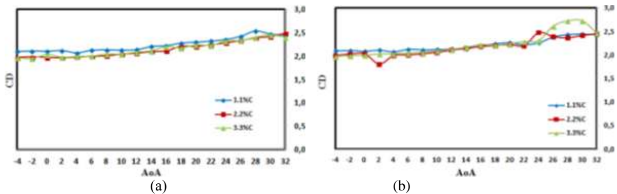
Figure 6. Comparison drag coefficient of variation tab heights versus angle of attach for (a) tab upper surface and (b) tab lower surface.
