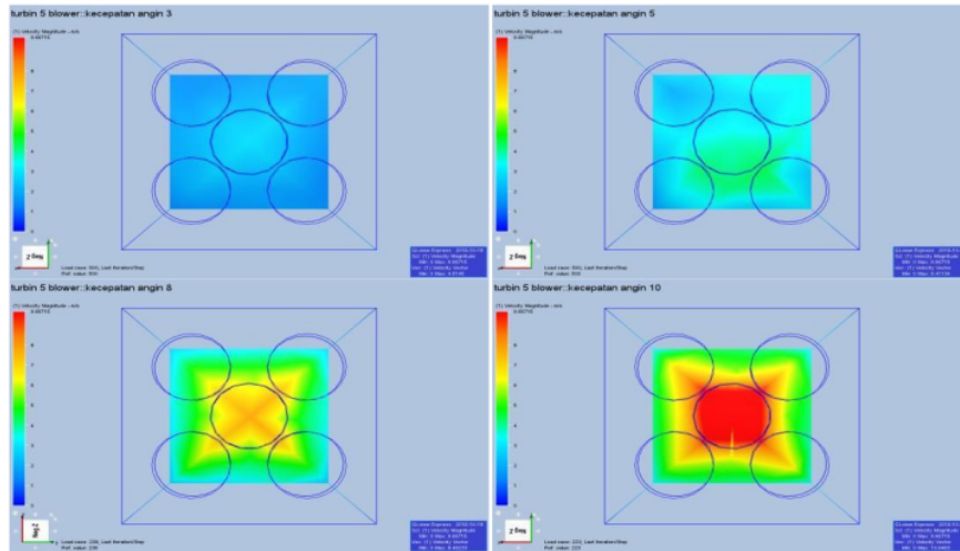
Figure 3. Distance on 2 meter rotor wind turbine position againt blower
