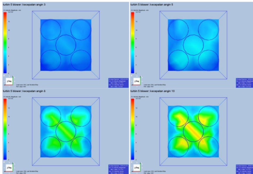
Figure 1. Distance on 1 meter rotor wind turbine position against blower
