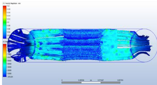
Figure 3. Velocity contour of biofluid
