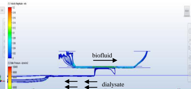
Figure 4. Route of biofluid in microchannel
