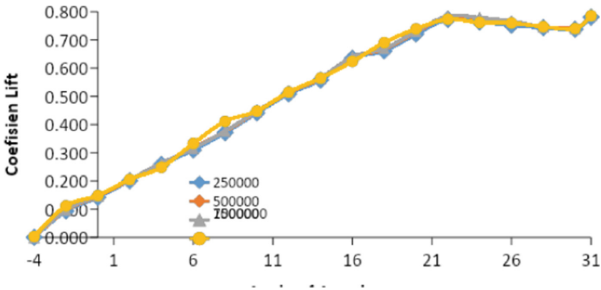
Fig. 2. Comparison lift coefficient versus angle of attack on variation Reynold Number.
