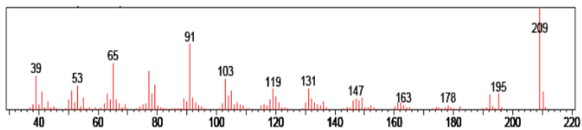
Gambar 5. Spektrum massa 4-allyl-2-metoksi-6-nitrofenol (2)
