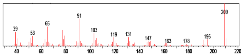
Gambar 2. Spektrum massa eugenol (1)
