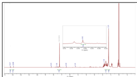
Figure 6. ^1\text{H-NMR} spectra of 1,3-dihydroxy-2-prenylxanthone
