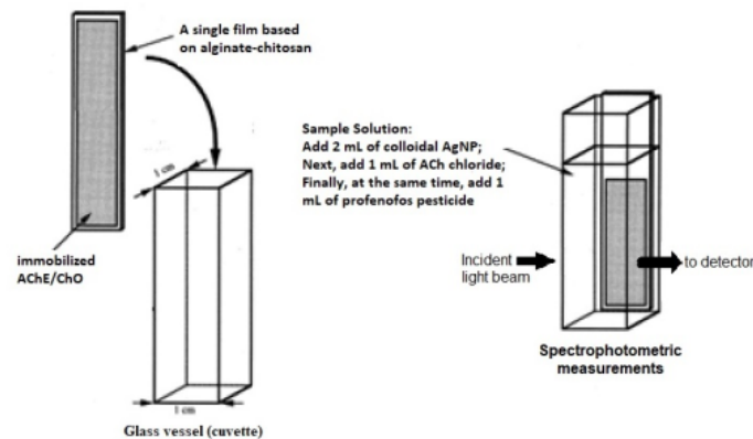
Fig. 1: Biosensor design
