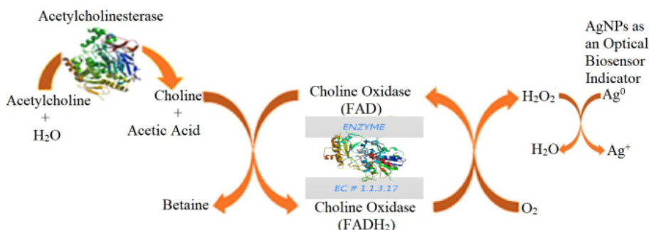
Fig. 2: Scheme of enzymatic reaction (AChE/ChO)
