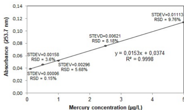
Figure 1. The Calibration Plot of Hg Measurement
