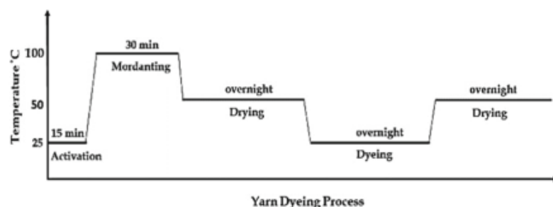
Fig. 1. Diagram of Yarn Dyeing Process
