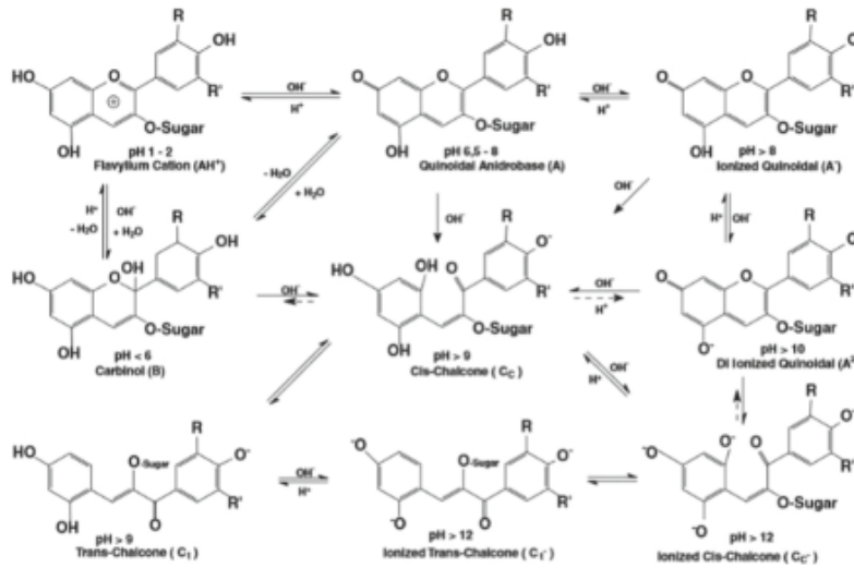
Fig. 2. Anthocyanin structure in pH-dependent speciation balance was suggested in previous studies [22]
