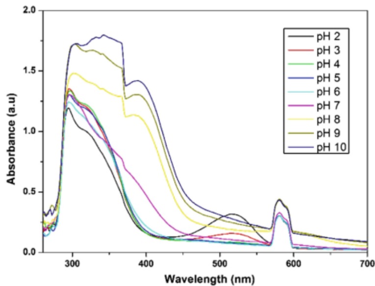
Fig. 3. Scanning of the wavelength of hanjuang leaves extract
