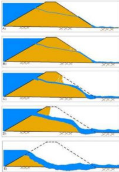
Gambar 3. Proses breach akibat piping (Hydrologic Engineering Center, 2014).
