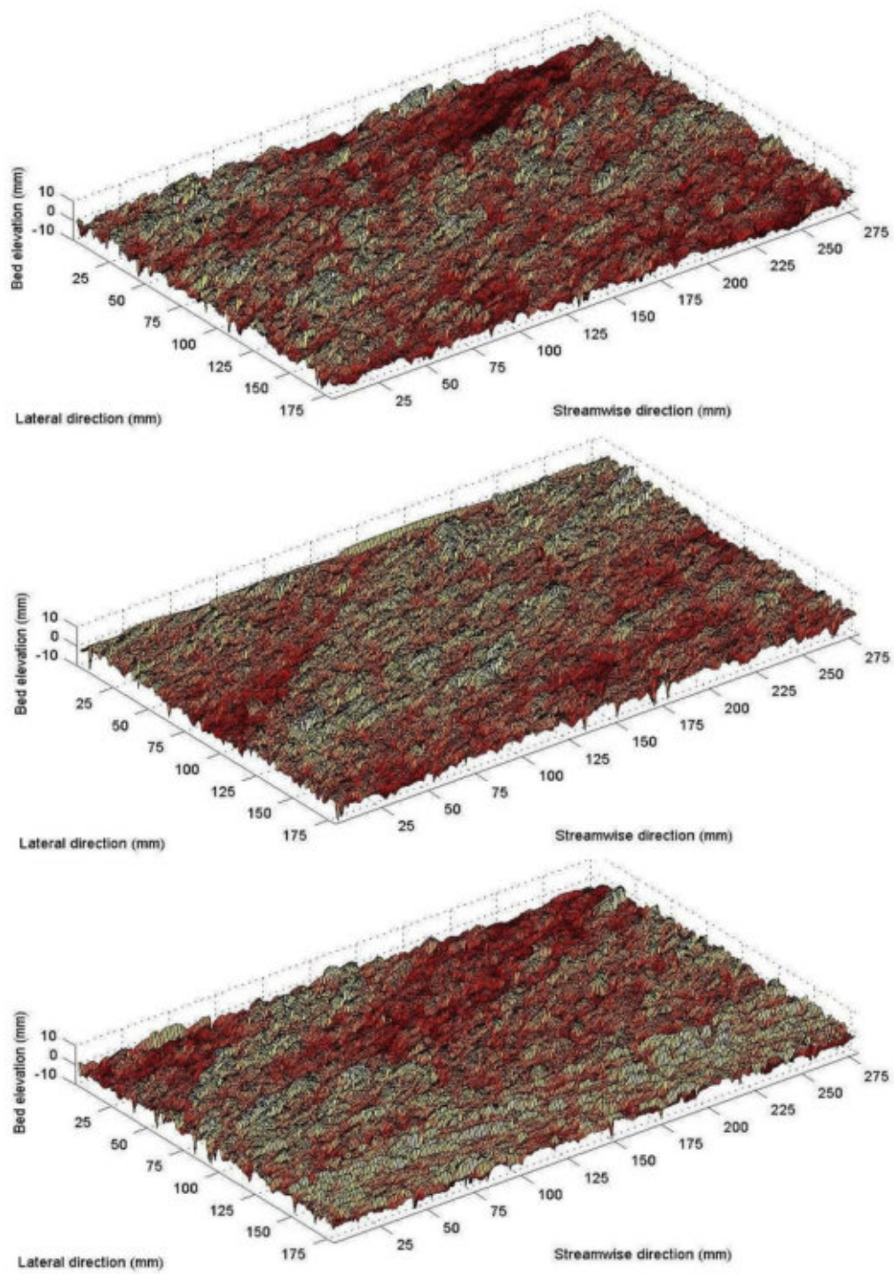
Figure 2. Bed surface topography of the measurement grid after stability test (from top to bottom picture are experiments 6H, 9H and 12H)
