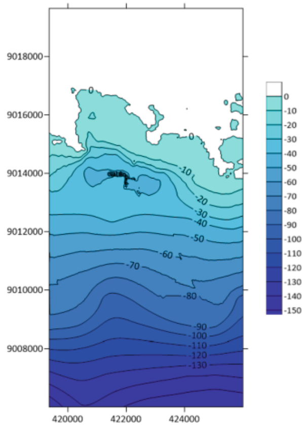
Fig. 3. The bathymetry map of Kuta Mandalika (analysis).
