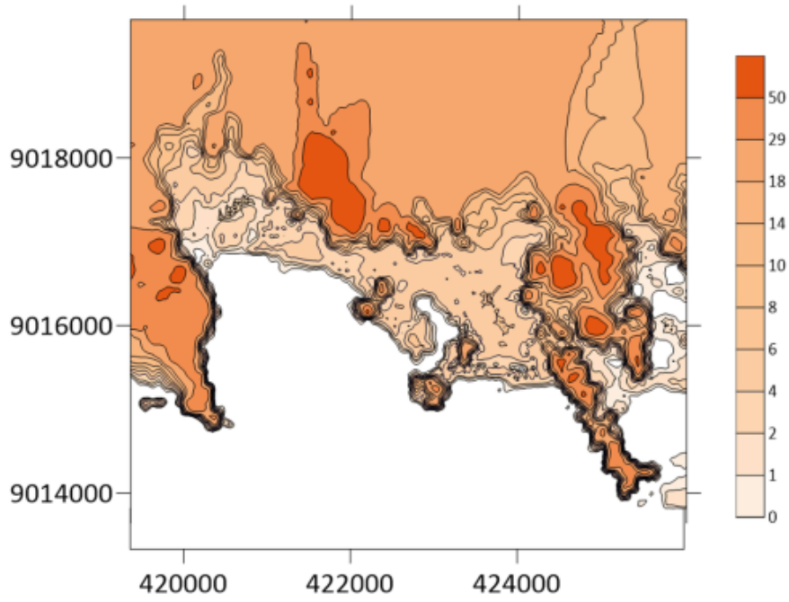
Fig. 2. The topography map of Kuta Mandalika (analysis)
