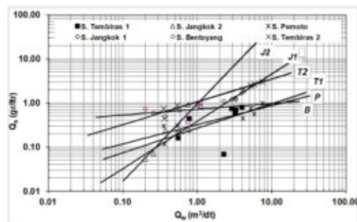
Fig. 7. Suspended sediment-flow discharge rating curve of six rivers in the upper course of Jangkok River
