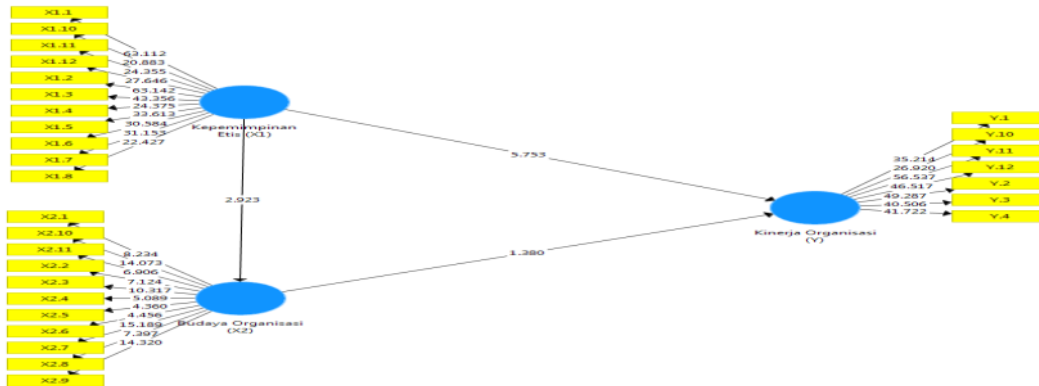
Figure 2. Hypothesis Test
