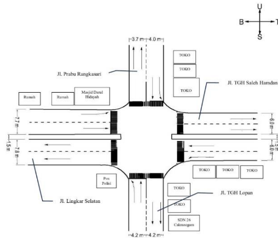
Gambar 3 Geometrik Simpang Dasan Cermen
