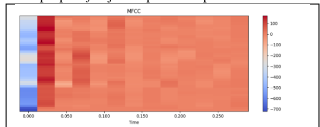
Gambar 7. Plotting MFCC
