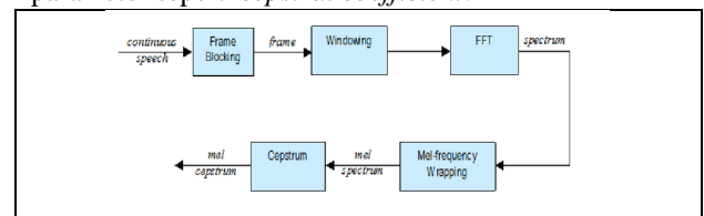
Gambar 1. Diagram Blok MFCC
