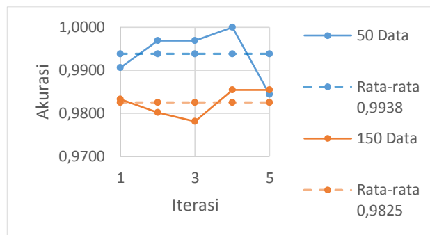
Gambar 12. Hasil Testing Overfitting
