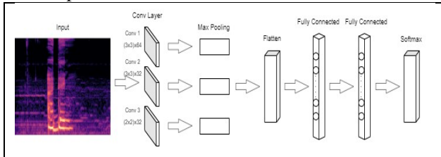
Gambar 8. Model CNN
