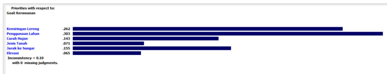
Gambar 2. Hasil Perhitungan AHP Expert Choice 11
